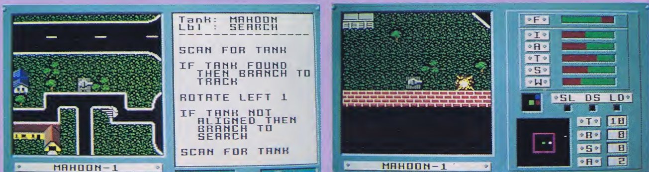
Above: In the testing module with trace mode on. This allows you to follow the tank's AI on screen and see what effect the instructions have on its behaviour (an essential thing to do prior to putting your tank in for evaluation, (Above Right)). That wait instruction seems to have paid dividends as the OSI tank takes a direct hit during the battlefield tests.
